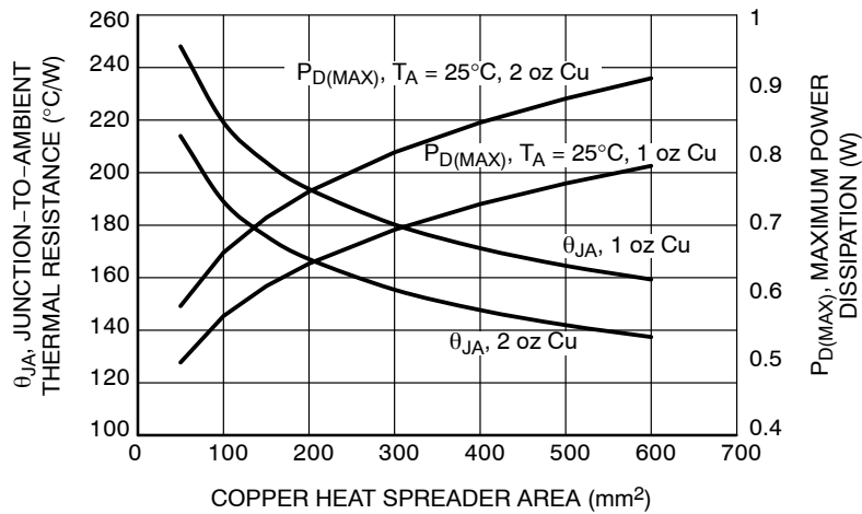
Figure 42. \theta_{JA} vs. Copper Area ( \mu\text{DFN4} )
