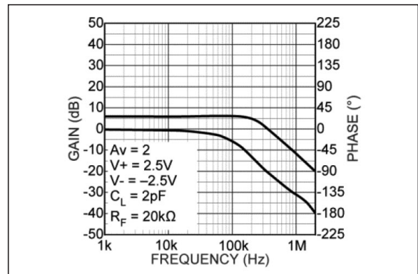
FIGURE 2-23: Gain Bandwidth and Phase Margin.
