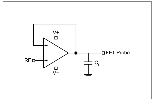
FIGURE 3-6: Test Circuit: 6 Closed-Loop Unity Gain Frequency Response Measurement.
