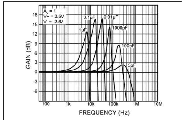
FIGURE 2-24: Closed-Loop Unity Gain Frequency Response.
