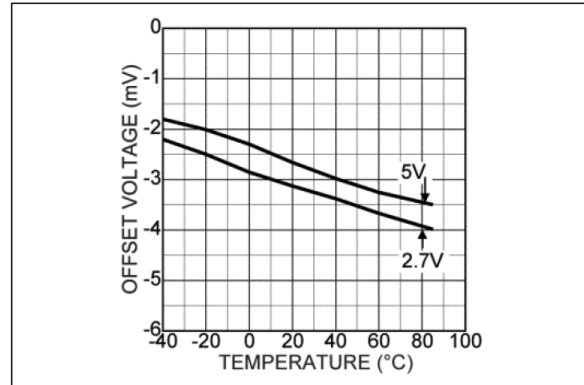
FIGURE 2-10: Offset Voltage vs. Temperature.
