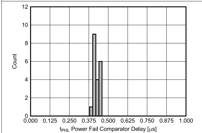
Figure 7-22. PFI to PFO ( t_{PHL} ) Delay Histogram for TPS3705-33 Devices at 25°C (Unit Count = 20)
