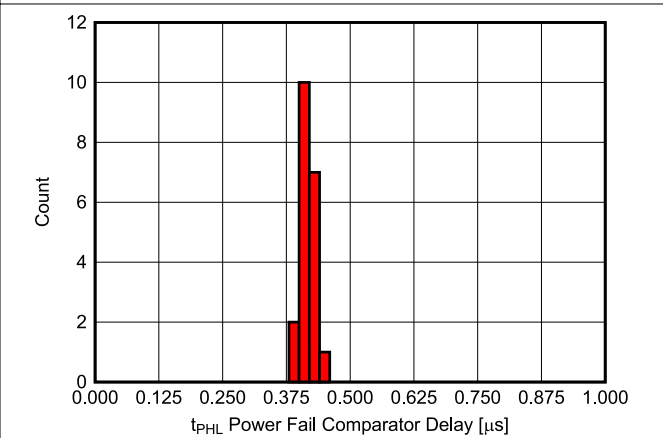
Figure 7-23. PFI to PFO ( t_{PHL} ) Delay Histogram for TPS3705-33 Devices at 125°C (Unit Count = 20)
