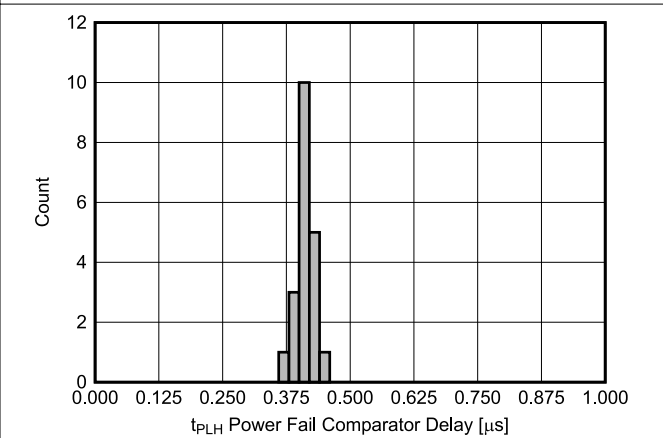
Figure 7-25. PFI to PFO ( t_{PLH} ) Delay Histogram for TPS3705-33 Devices at 25°C (Unit Count = 20)
