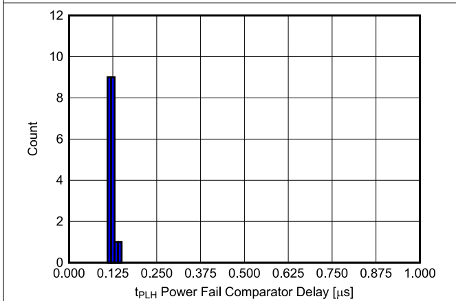
Figure 7-24. PFI to PFO ( t_{PLH} ) Delay Histogram for TPS3705-33 Devices at -40°C (Unit Count = 20)
