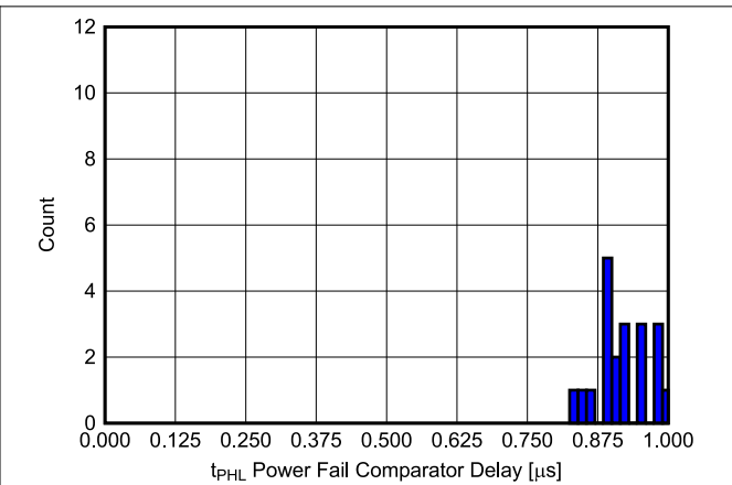
Figure 7-21. PFI to PFO ( t_{PHL} ) Delay Histogram for TPS3705-33 Devices at -40°C (Unit Count = 20)
