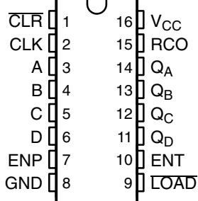
SN54LV163A . . . J OR W PACKAGE SN74LV163A . . . D, DB, DGV, NS, OR PW PACKAGE (TOP VIEW)
