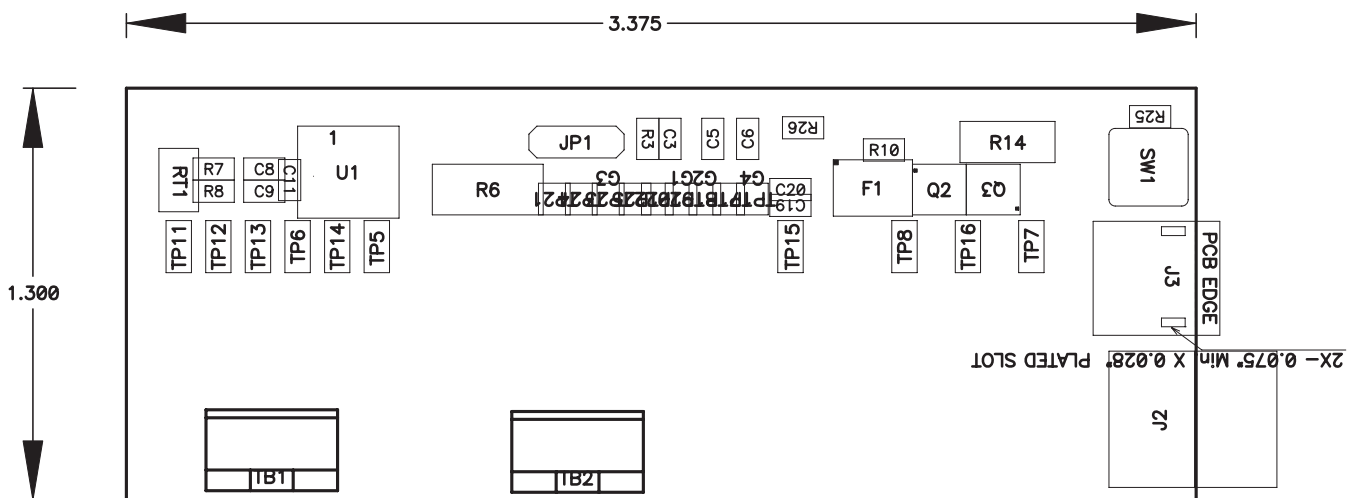
Figure 2. Top Assembly
