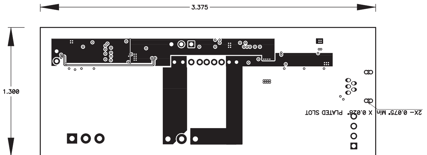
Figure 5. Internal Layer 2
