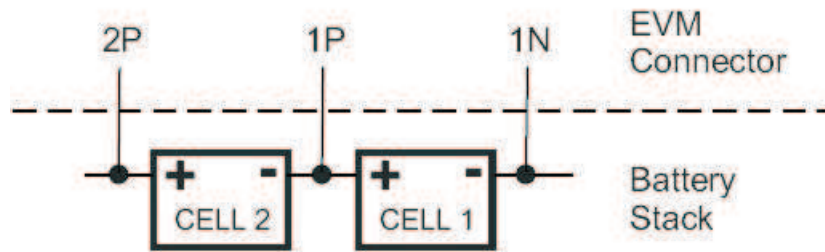
Figure 14. Connection Sequence
