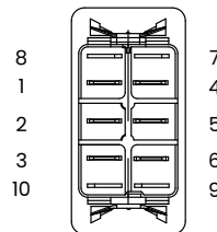
BOTTOM VIEW TERMINAL ARRANGEMENT 10 TERMINAL BASE
