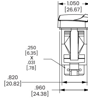
10 TERMINAL BASE W/O BARRIERS
