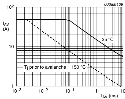
Fig 5. Single-shot avalanche rating; avalanche current as a function of avalanche period
