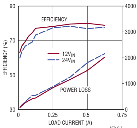
Efficiency and Power Loss, V OUT = -12V
