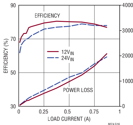
Efficiency and Power Loss, V OUT = -8V
