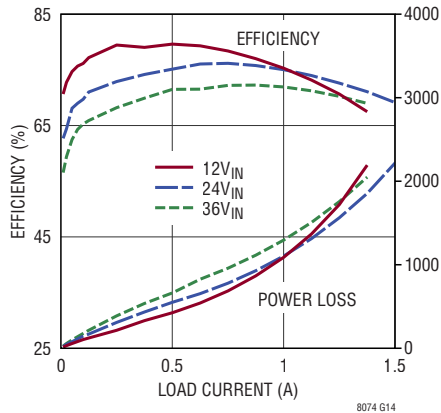
Efficiency and Power Loss, V OUT = -3.3V
