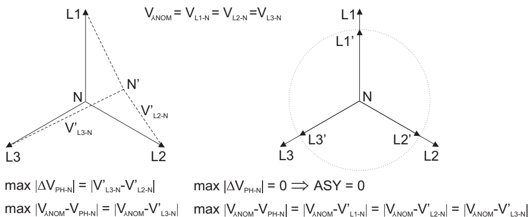
Fig. 2 Phase-neutral monitoring
