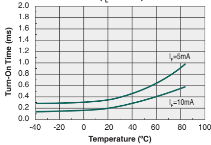
Turn-On Time vs. Temperature ( I_L=80mA )
