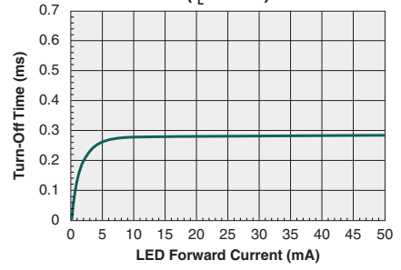
Turn-Off Time vs. LED Forward Current ( I_L=80mA )
