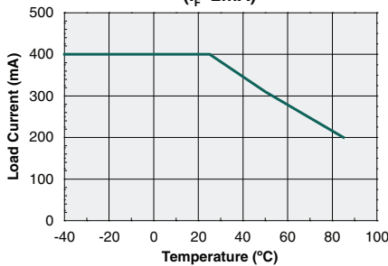
Maximum Load Current vs. Temperature ( I_F=2mA )
