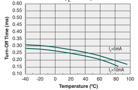
Turn-Off Time vs. Temperature ( I_L=80mA )
