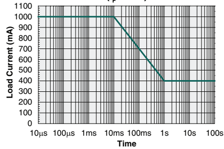
Energy Rating Curve ( I_F=2mA )
