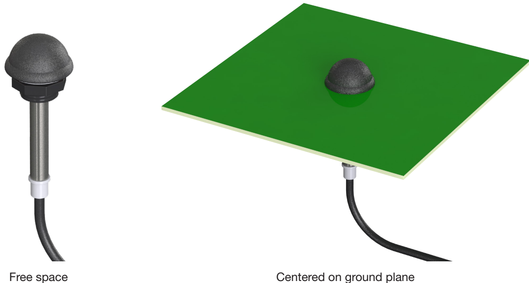
Figure 3. ANT-DB1-WRT-ccc Test Orientations
