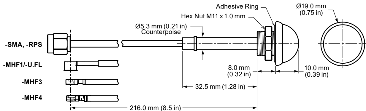
Figure 1. ANT-DB1-WRT Antenna Dimensions
