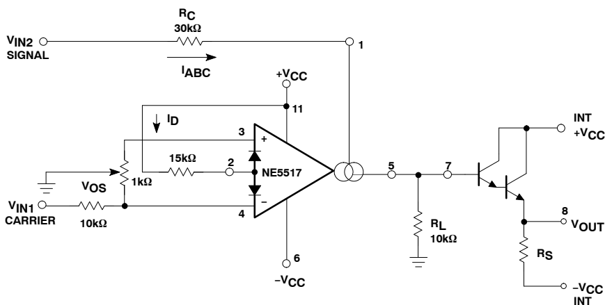
Figure 25. Amplitude Modulator
