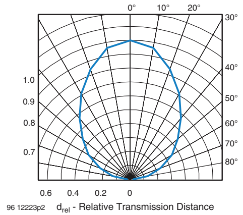
Fig. 11 - Horizontal Directivity
