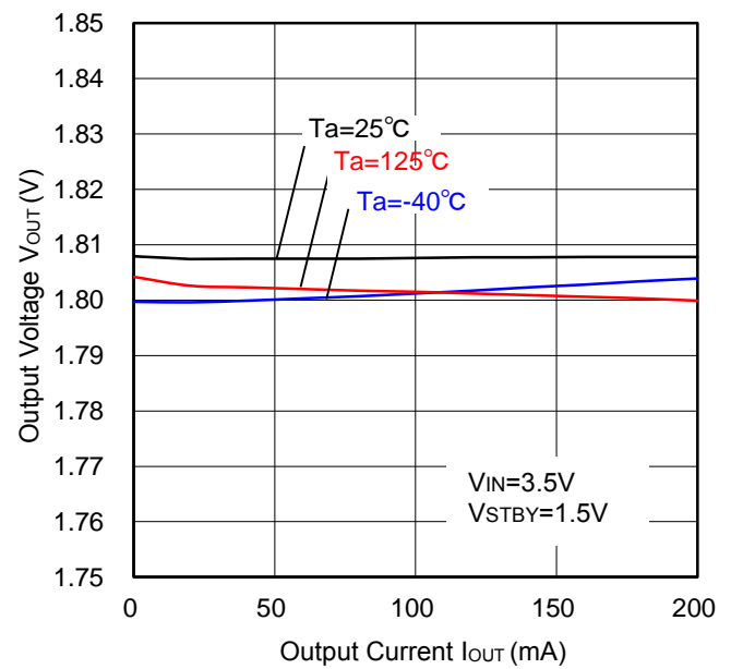
Figure 6. Load Regulation
