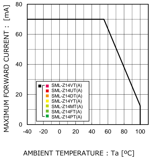
Fig.4 Derating
