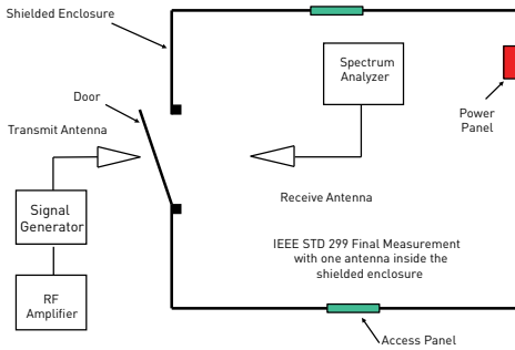
Figure 3-2. IEEE STD 299
