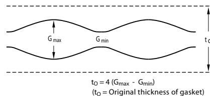
Figure 1-10: Gasket Deflection Along a Flange
