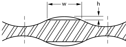
Figure 1-16. Unfilled Slot is Free to Radiate When Spacing is Equal to 1/2 Wavelength
