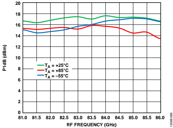
Figure 65. Input P1dB vs. RF Frequency at Various Temperatures, LO = 2 \text{ dBm} , IF = 1000 \text{ MHz} , LSB
