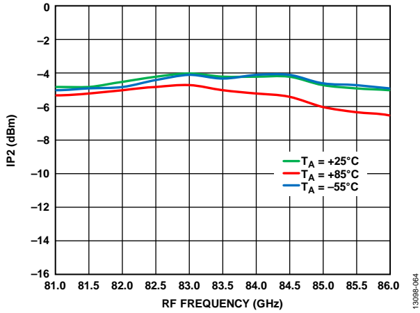
Figure 63. Input IP2 vs. RF Frequency at Various Temperatures, I_{FIN} = 5 \text{ dBm} , LO = 2 \text{ dBm} , IF = 1000 \text{ MHz} , LSB
