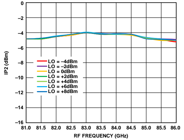
Figure 66. Input IP2 vs. RF Frequency at Various LO Powers, I_{FIN} = 5 \text{ dBm} , IF = 1000 \text{ MHz} , LSB
