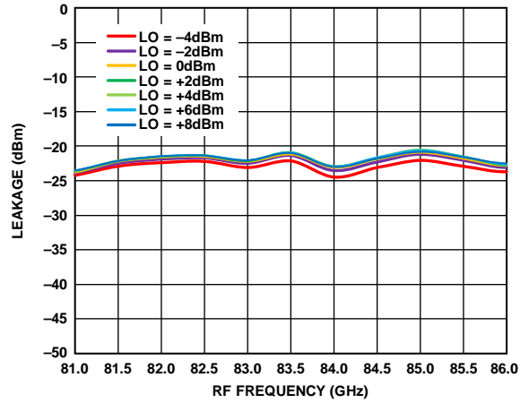
Figure 67. 6 \times LO Leakage at RFOUT vs. RF Frequency at Various LO Powers, I_{FIN} = 5 \text{ dBm} , IF = 1000 \text{ MHz} , LSB
