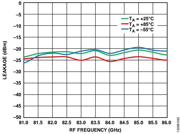
Figure 64. 6 \times LO Leakage at RFOUT vs. RF Frequency at Various Temperatures, I_{FIN} = 5 \text{ dBm} , LO = 2 \text{ dBm} , IF = 1000 \text{ MHz} , LSB
