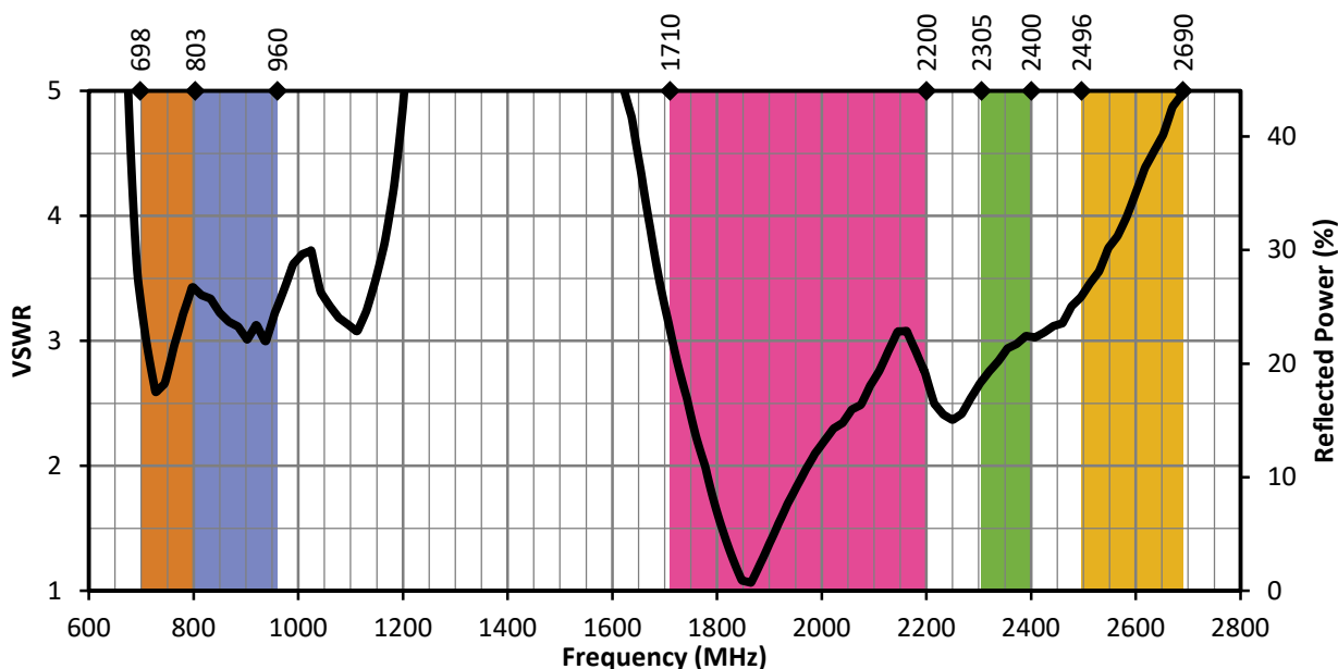
Figure 1. SP610 VSWR with Frequency Band Highlights
