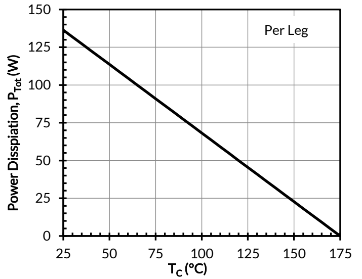
Figure 4. Power dissipation
