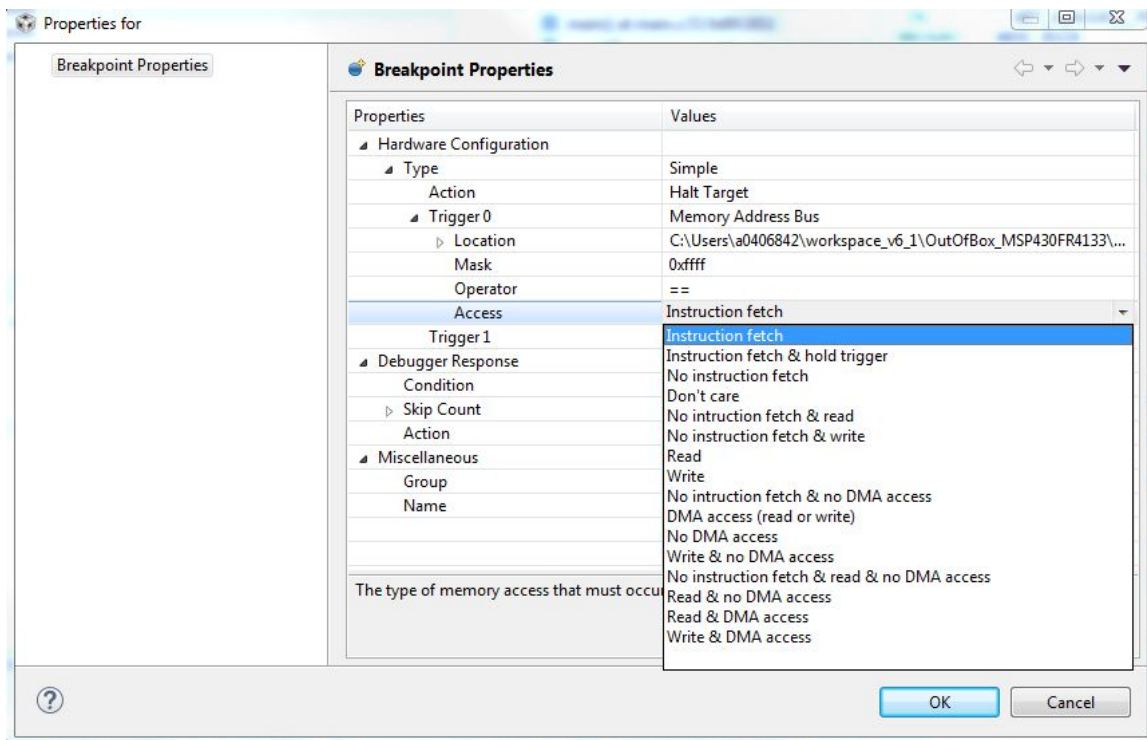
Figure 3-2. Breakpoint Properties
