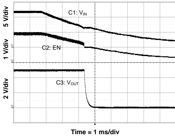
Figure 18. Shutdown Relative to V_{IN}
