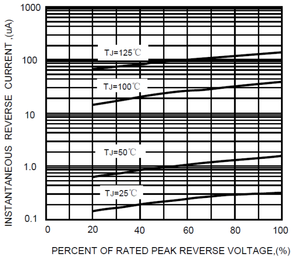
FIG.3-TYPICAL REVERSE CHARACTERISTICS
