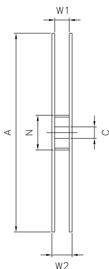
Reel dimensions in mm
