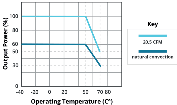
TEMPERATURE DERATING CURVE VMS-350C-12 (full load 300W with 20.5 CFM)
