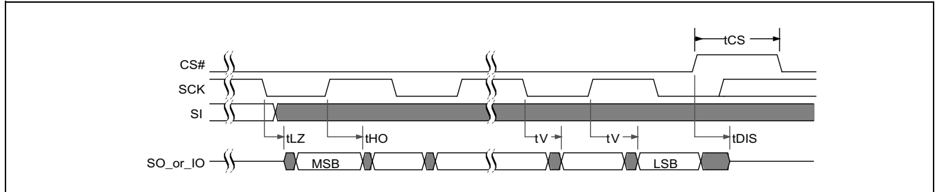
Figure 37 SPI DDR output timing
