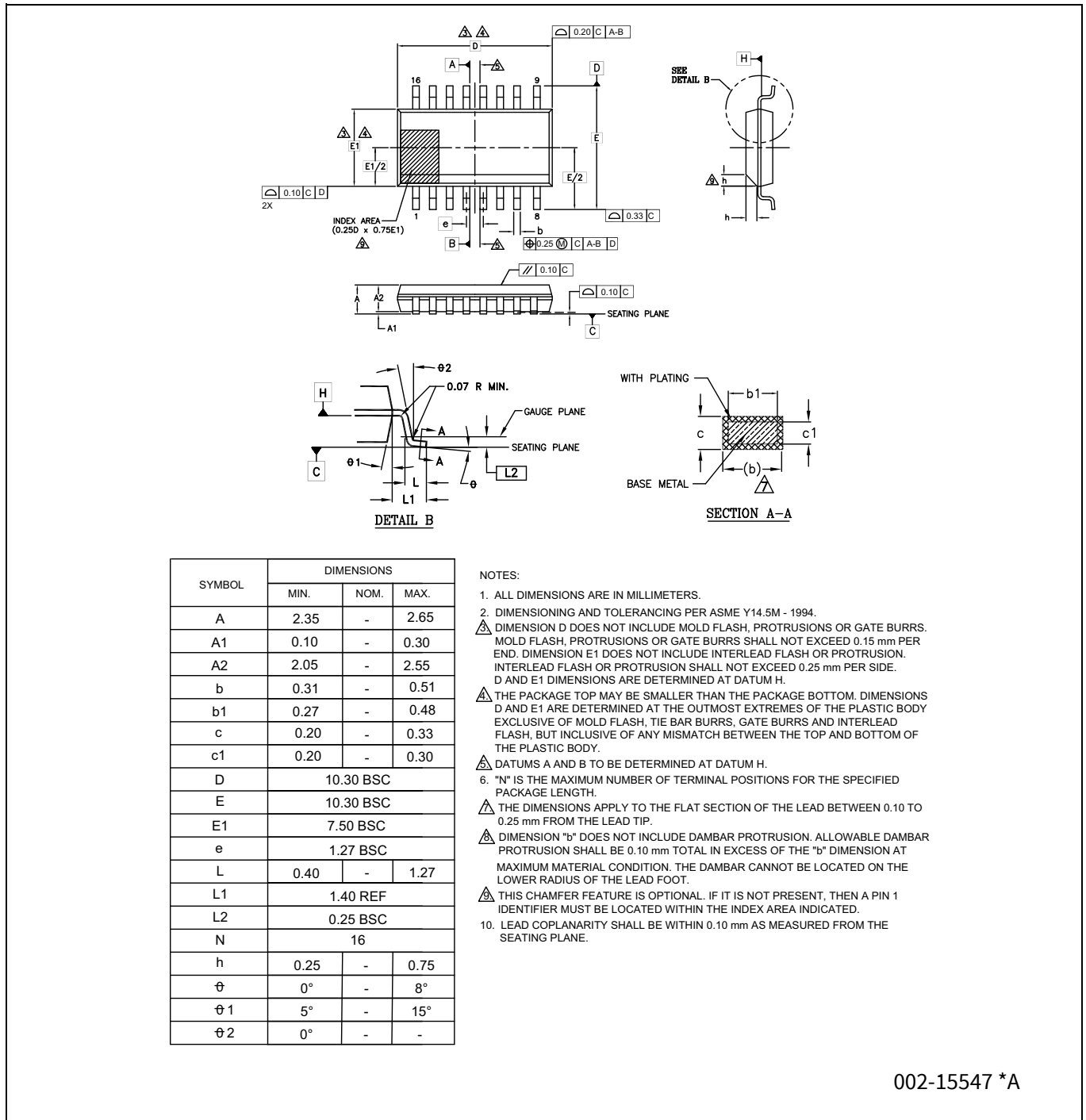
Figure 150 SOIC 16-lead, 300-mil body width (S03016)
