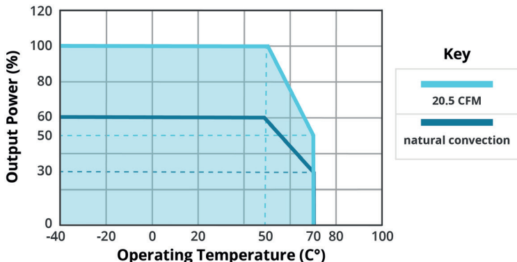
TEMPERATURE DERATING CURVE (full load 300W with 20.5 CFM) VOF-350C-12
