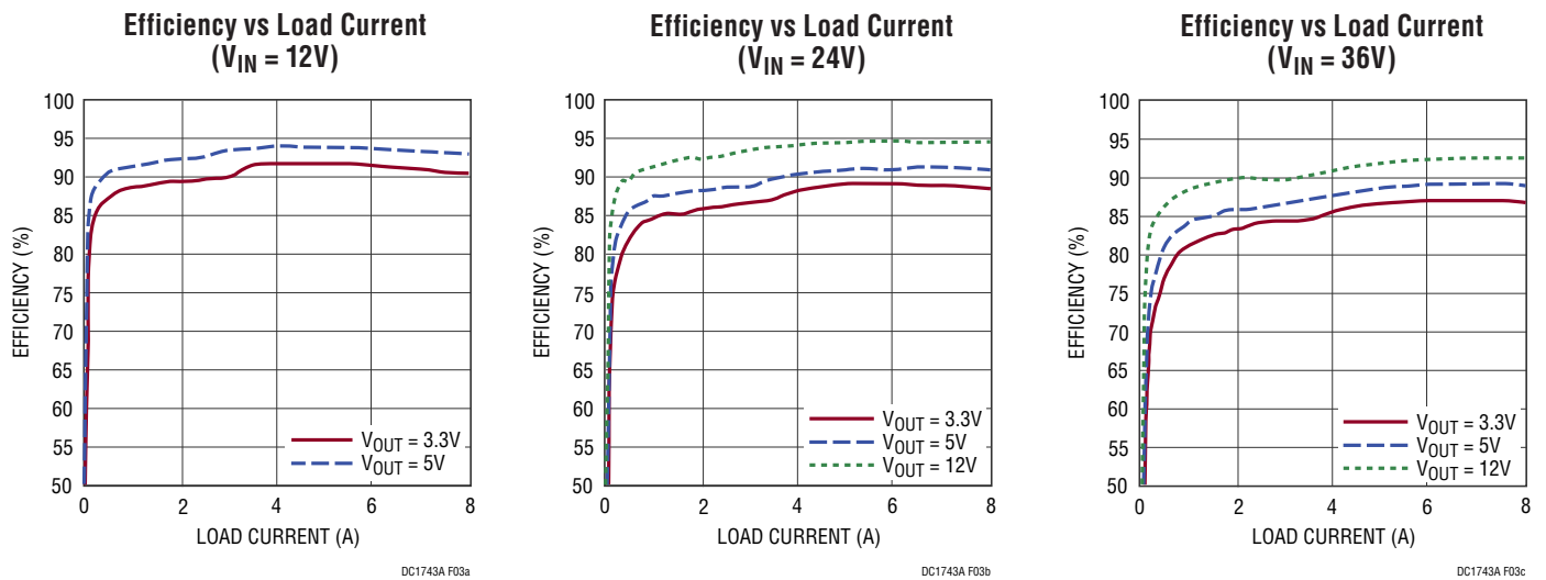
Figure 3. Measured DC1743A Efficiency at Different V_{IN} and V_{OUT} (DCM Mode Enabled)
