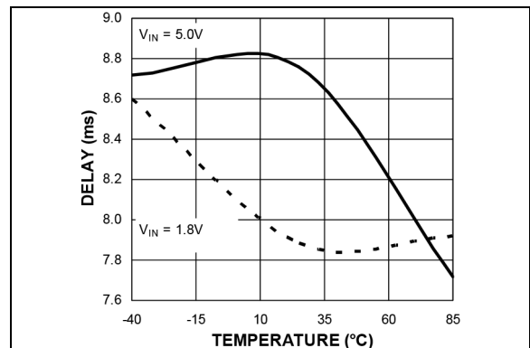
FIGURE 2-30: OGI Delay vs. Temperature.
