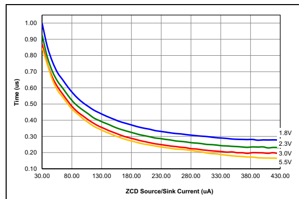
FIGURE 36-102: ZCD Pin Response Timer over Current, Typical Measured Values from -40^\circ\text{C} to 125^\circ\text{C} .
