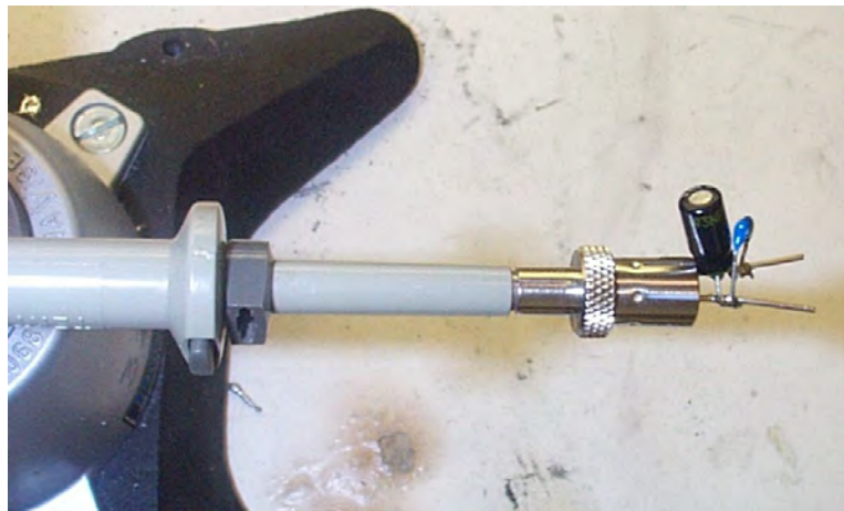
Figure 47 – Oscilloscope Probe with Probe Master 4987BA BNC Adapter (Modified with Wires for Probe Ground for Ripple measurement and Two Parallel Decoupling Capacitors Added).
