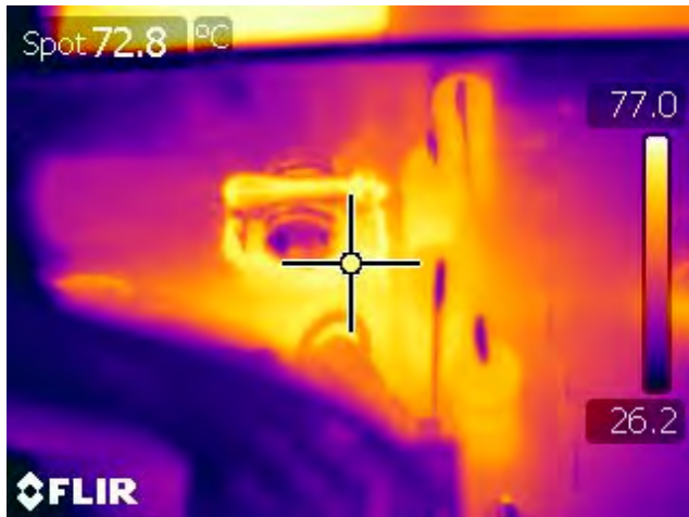
Figure 67 – Output Rectifier (D11), 115 VAC Input, 100% Load, Room Temperature.
