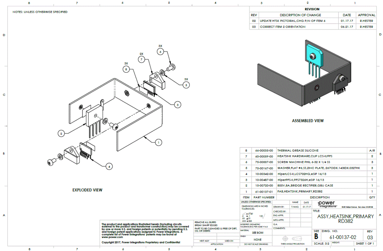
Figure 20 – RD-382 Primary Heat Sink Assembly.
