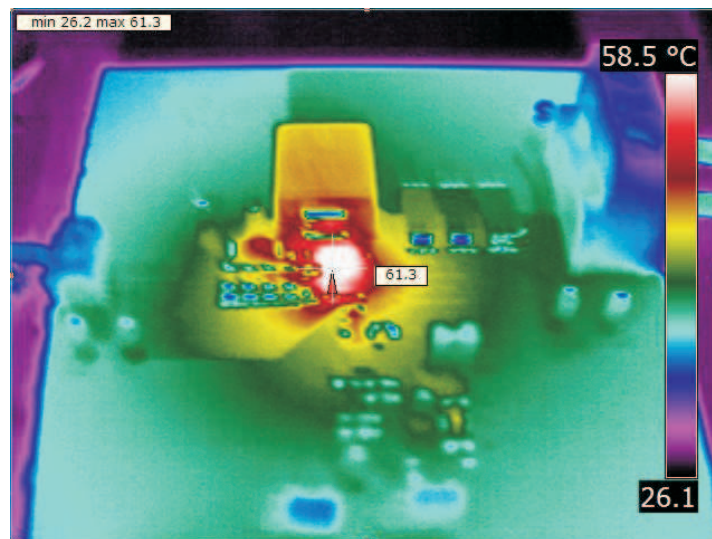
Figure 12. CSD86350Q5DEVM-604 Thermal Image
