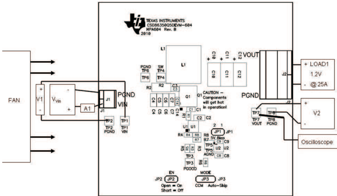
Figure 2. CSD86350Q5DEVM-604 Recommended Test Set-Up
