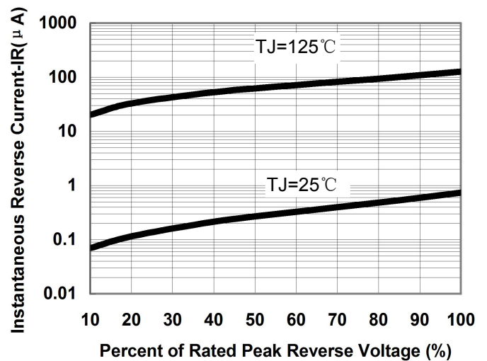
Fig.2-Typical Reverse Characteristics
