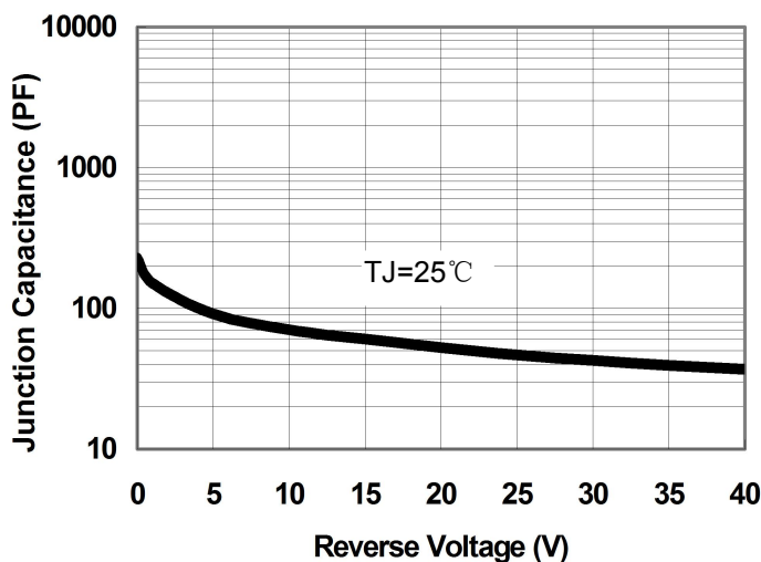
Fig.1-Typical Junction Capacitance
