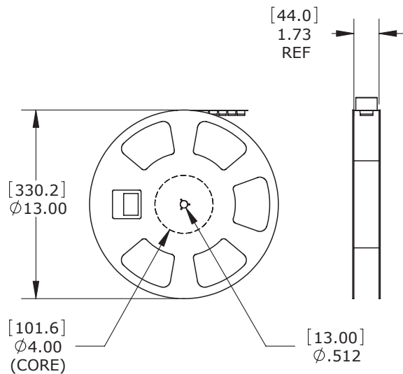
REEL INFORMATION (250 UNITS PER REEL)
