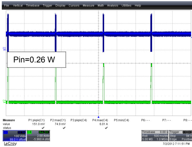
Figure 55 – Short-Circuit, 90 VAC. Upper: V_{DS} , 100 V / div. Lower: 5 V_{LOAD} , 500 ms, 2 A / div.
