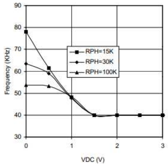
Graph 4. Frequency vs V DC (IR2156)
