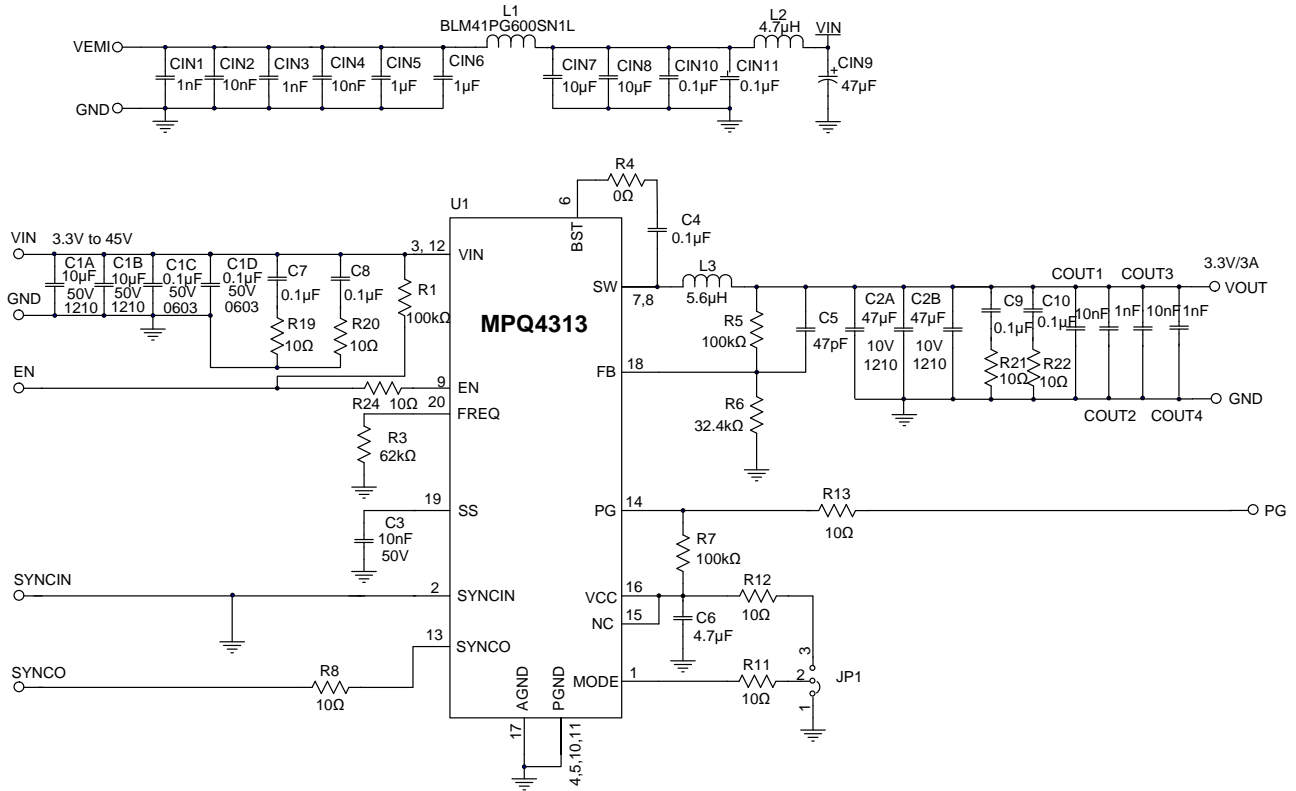
Figure 13: V OUT = 3.3V, f sw = 470kHz with EMI Filters
