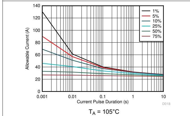
Figure 8-8. Maximum Repetitive Pulsed Current vs. Pulse Duration
