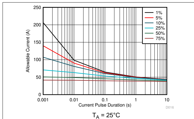
Figure 8-6. Maximum Repetitive Pulsed Current vs. Pulse Duration
