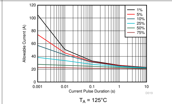
Figure 8-9. Maximum Repetitive Pulsed Current vs. Pulse Duration
