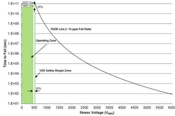
Figure 9-1. Insulation Lifetime
