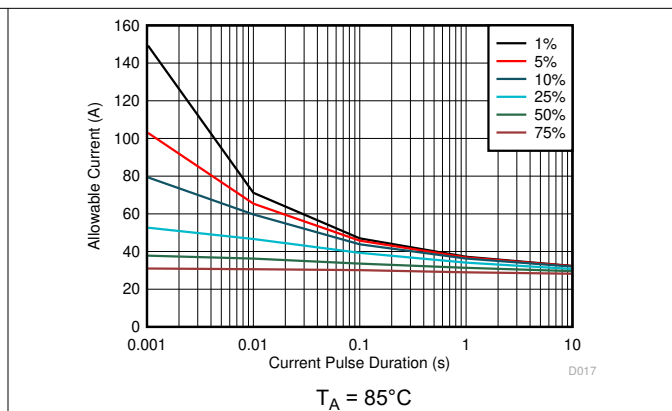
Figure 8-7. Maximum Repetitive Pulsed Current vs. Pulse Duration
