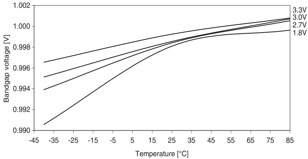
Figure 38-58. ADC/DAC Internal 1.0V reference vs. temperature.
