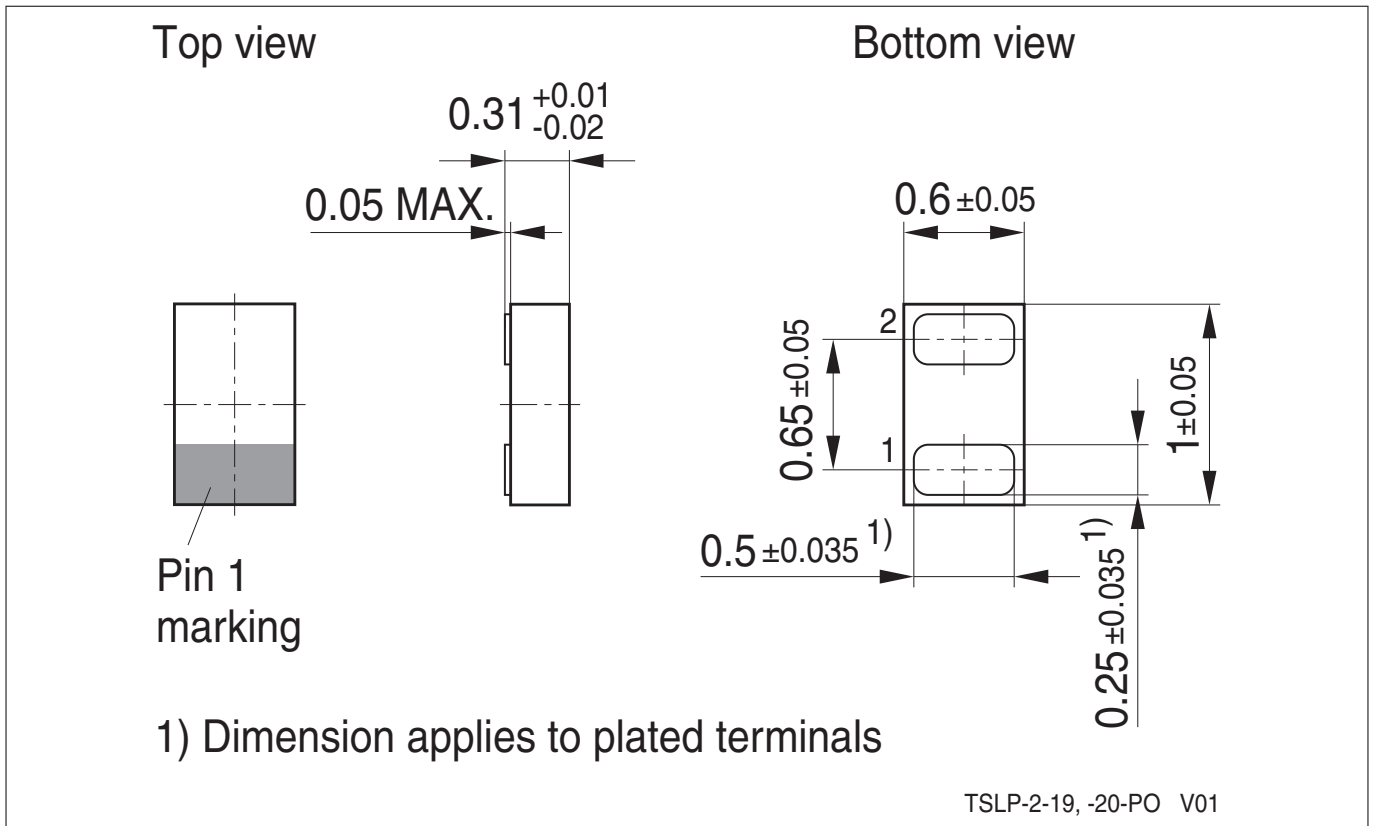
Figure 9 TSLP-2-20 package
