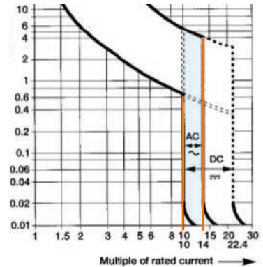
K Curve
