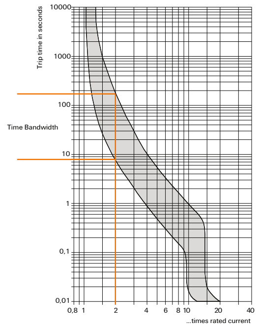
D Curve
