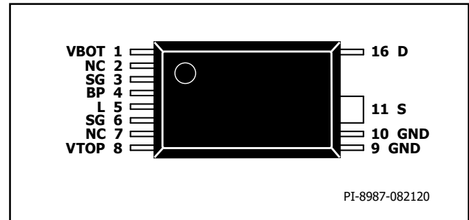
Figure 5. Pin Configuration.
