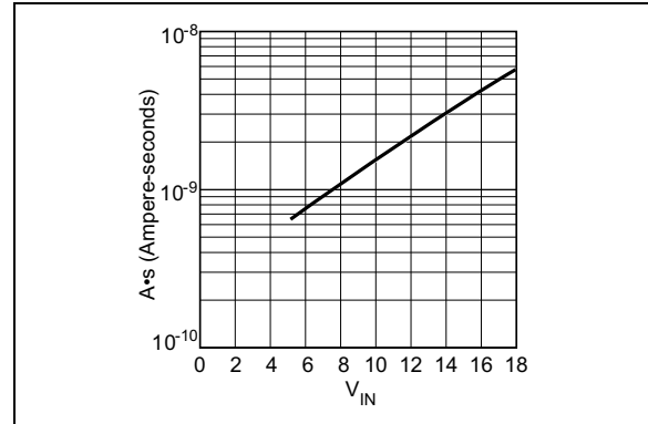
FIGURE 4-1: Crossover Energy Loss.
