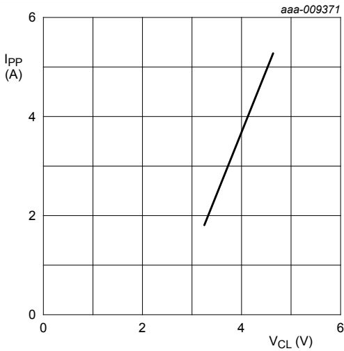
Figure 11. Dynamic resistance with positive clamping; typical values
