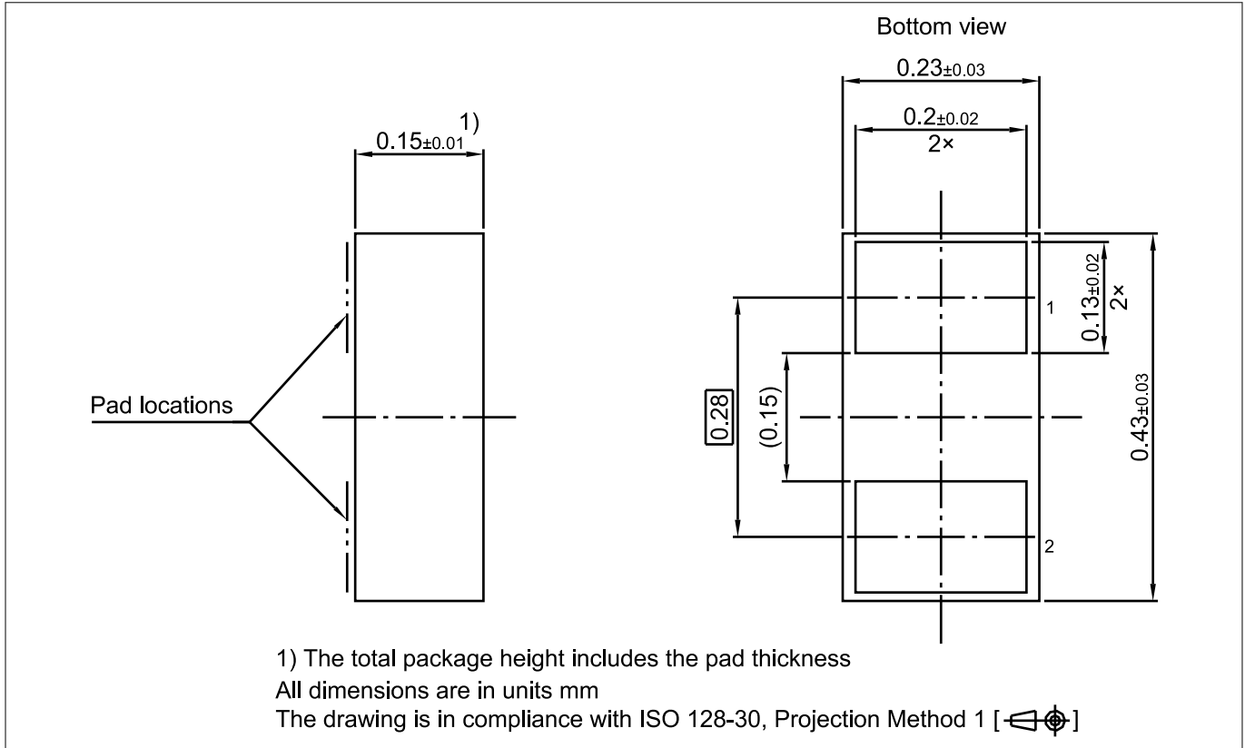
Figure 13 WLL-2-2 package
