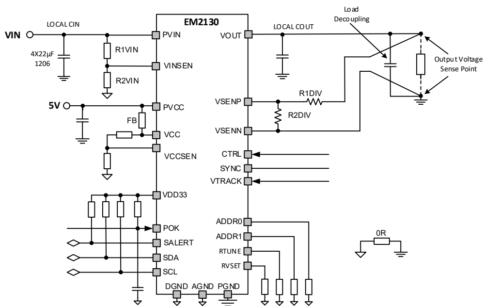
Figure 16: Recommended Application Circuit
