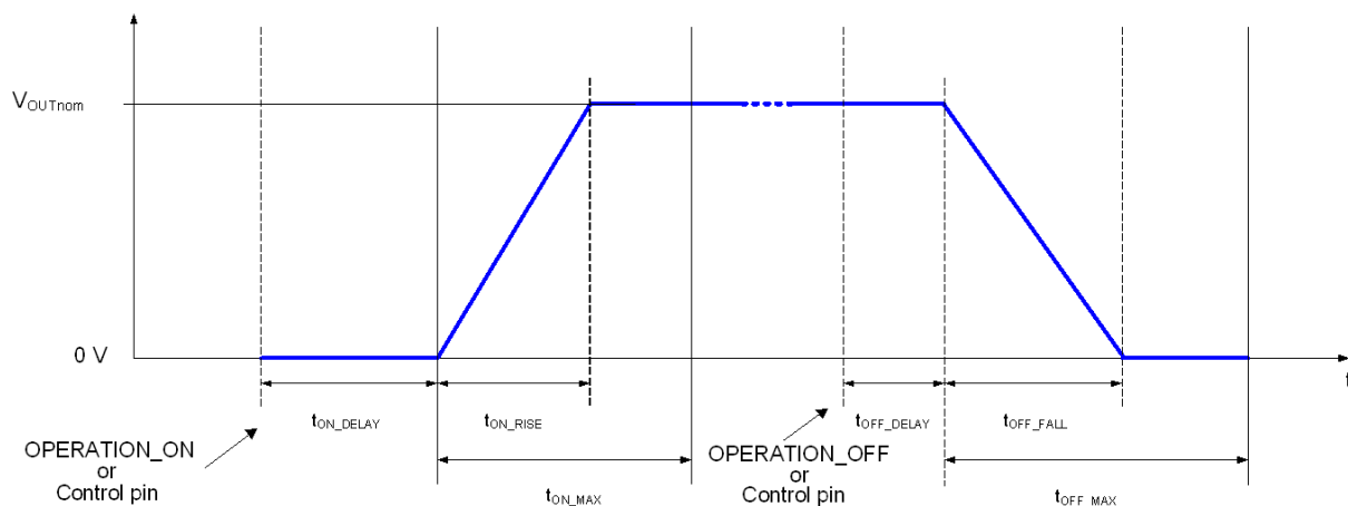
Figure 6: Power Sequencing
