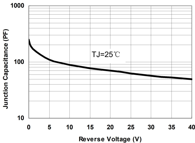
Fig.1-Typical Junction Capacitance
